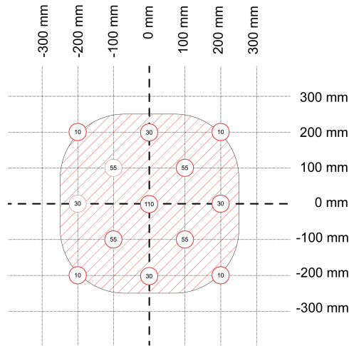
Beleuchtungsstärke in Lux in 1,5 m Abstand Illumination level in Lux at a distance of 1.5 m
